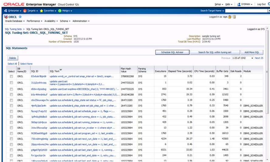
FIGURE 9.26 SQL Tuning Advisor results
