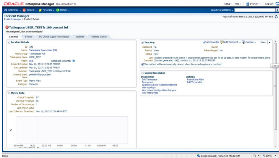
FIGURE 10.3 Tablespaces
